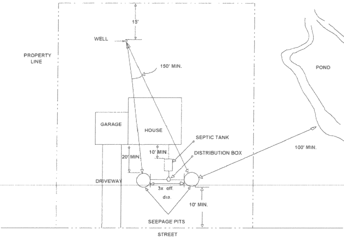
FIGURE 2 SEEPAGE PIT SEPARATION REQUIREMENTS
