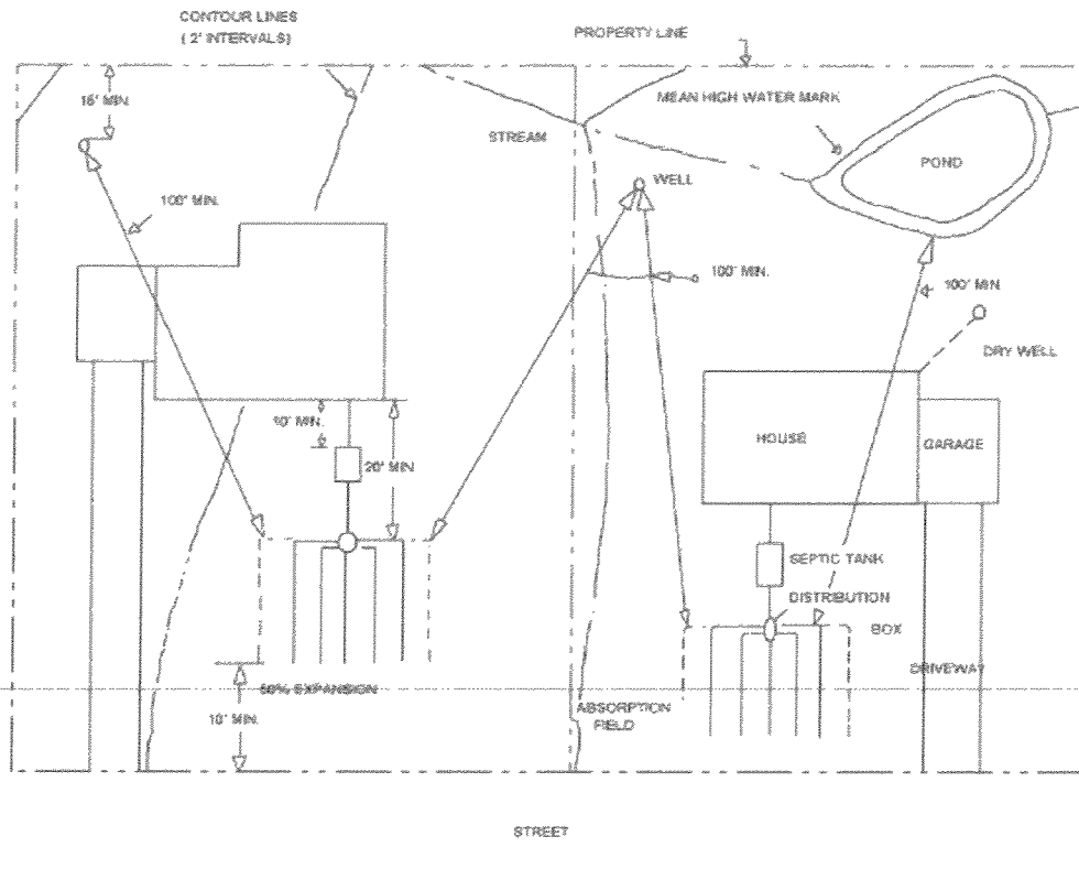
FIGURE 1 ABSORPTION FIELD SEPARATION REQUIREMENTS
